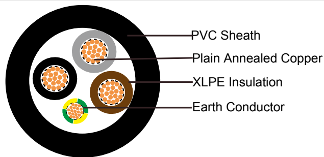
3 Cores+1 Core Earth Conductor
